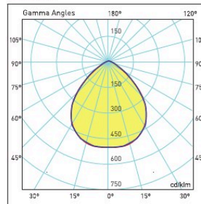
90° Lens
