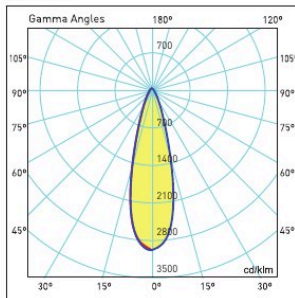
30° Lens
