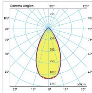
60° Lens
